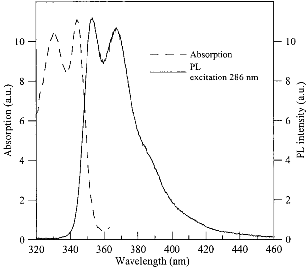
Figure 3. Absorption and photoluminescence spectra of R10EPK thin film at room temperature. PL spectrum measured after excitation at 286 nm.
